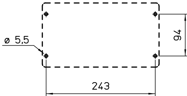
Fixing holes
